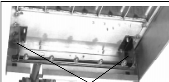
Figure 3 - Burner Rack Brackets at the Rear of the Heater
