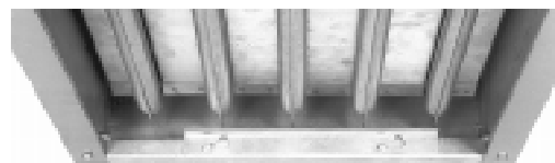
Figure 2 - Location of burner rack support as it was factory-installed on the inside front of the heater (Support was removed when the heater was disassembled; screws should be loosened but still in place.)
