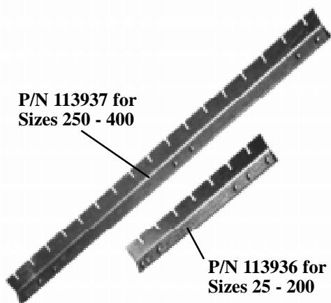
Figure 1 - Re-Designed Burner Rack Supports
