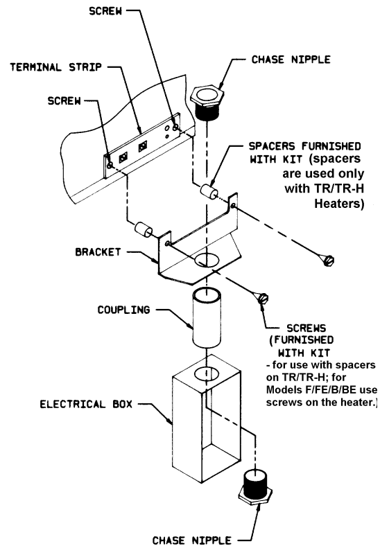
Figure 25 (Designed only for Models F, FE, B, BE, TR, and TR-H -- does not include thermostat)
